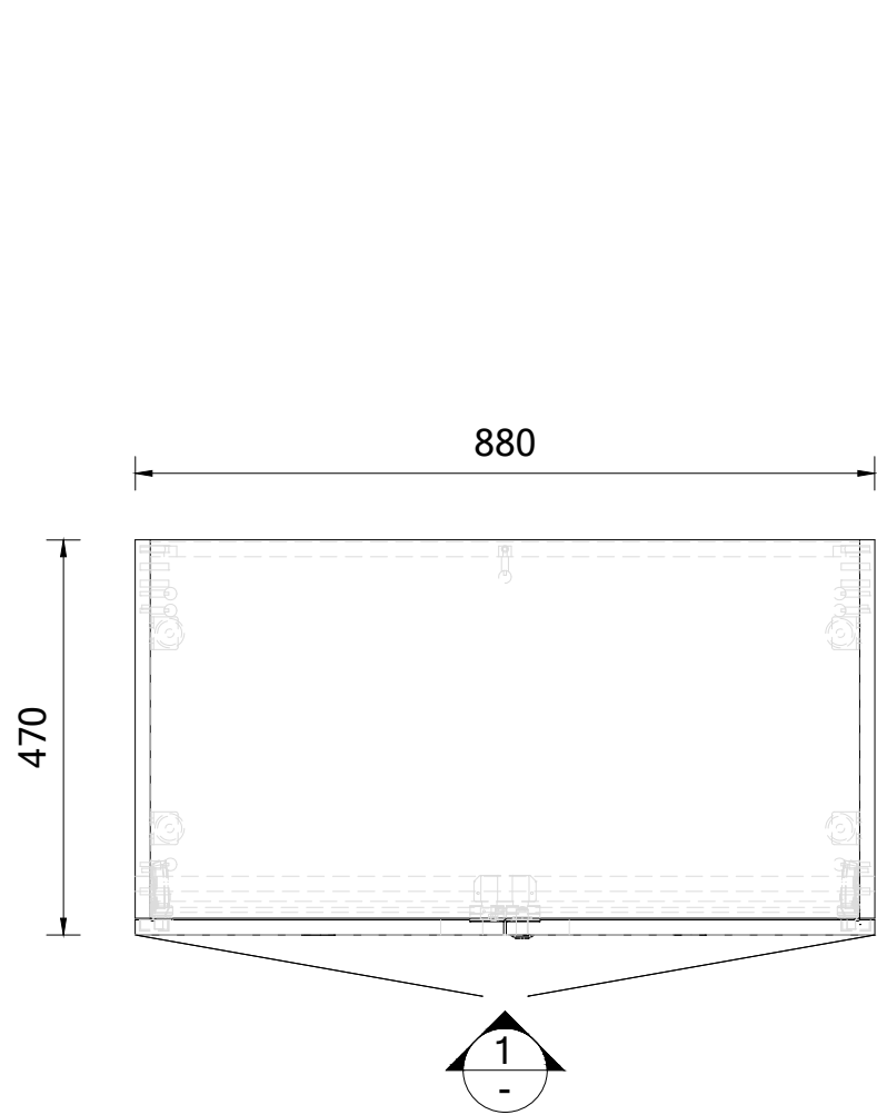
Plan View REC65
