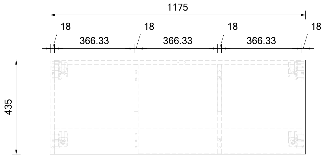
Plan View REB52
